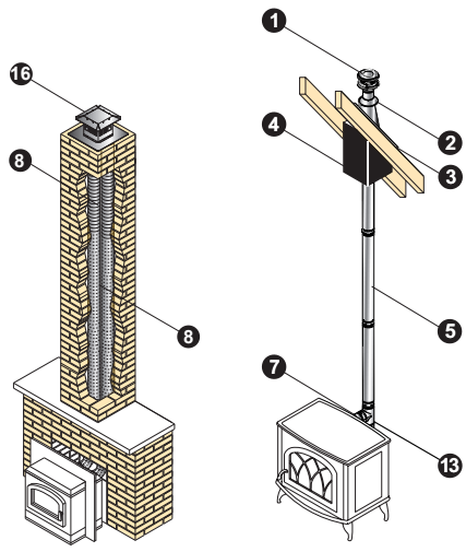
Co-Linear SS Flex Installation for Pellet Inserts
