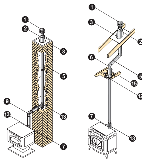
Masonry Chimney Relining with Rigid Pipe
